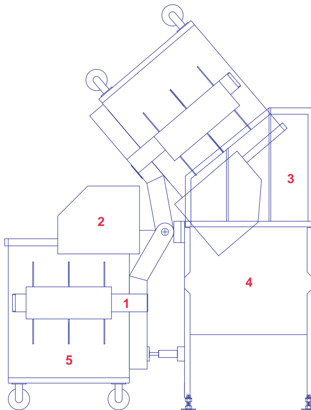
1. Cart tipper frame 2. Cart tipper waste chute 3. Feedram hopper waste chute 4. Feedram automatic loader 5. Waste Cart
